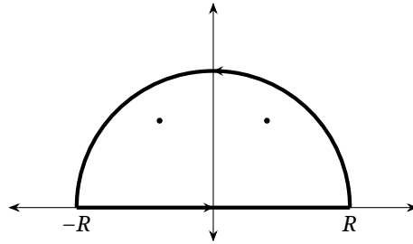
Figure 1: Contour in the upper half-plane, with the two points denoting the two simple poles of f(z) in the upper half-plane.
